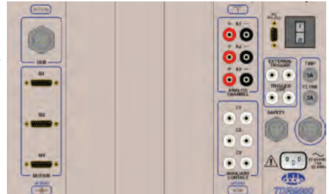
Figure 3. Minimum Configuration for Circuit Breakers with three Motion Channels, three Analog Channels, and three Auxiliary Contact Channels
